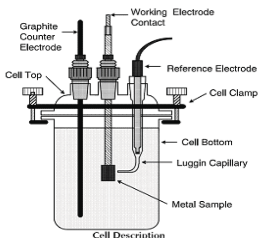
Fig (2). Schematic representation of a similar corrosion cell used for testing [13].
