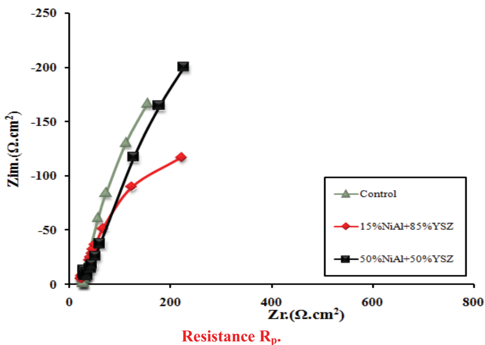
Fig. (5) Nyquist diagrams of impedance spectrum for control (uncoated) and NiAl+YSZ coated carbon steel in crude oil .
