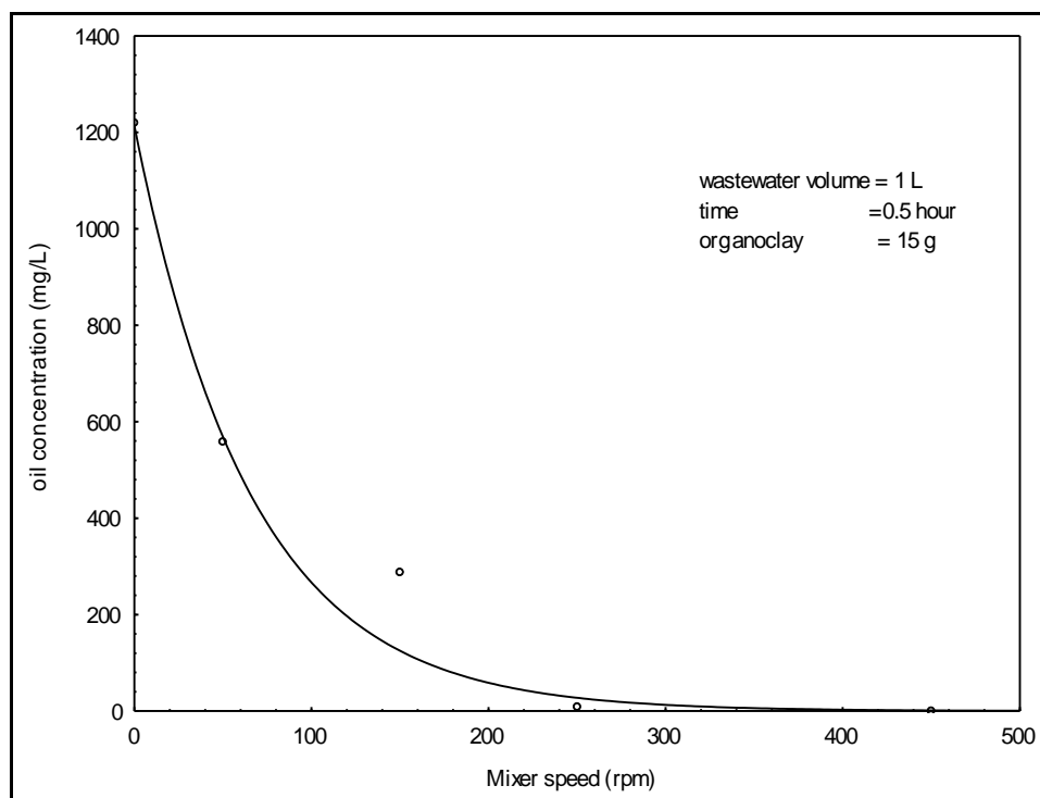
Fig. (11) Effect of mixer speed on oil removal using organoclay.
