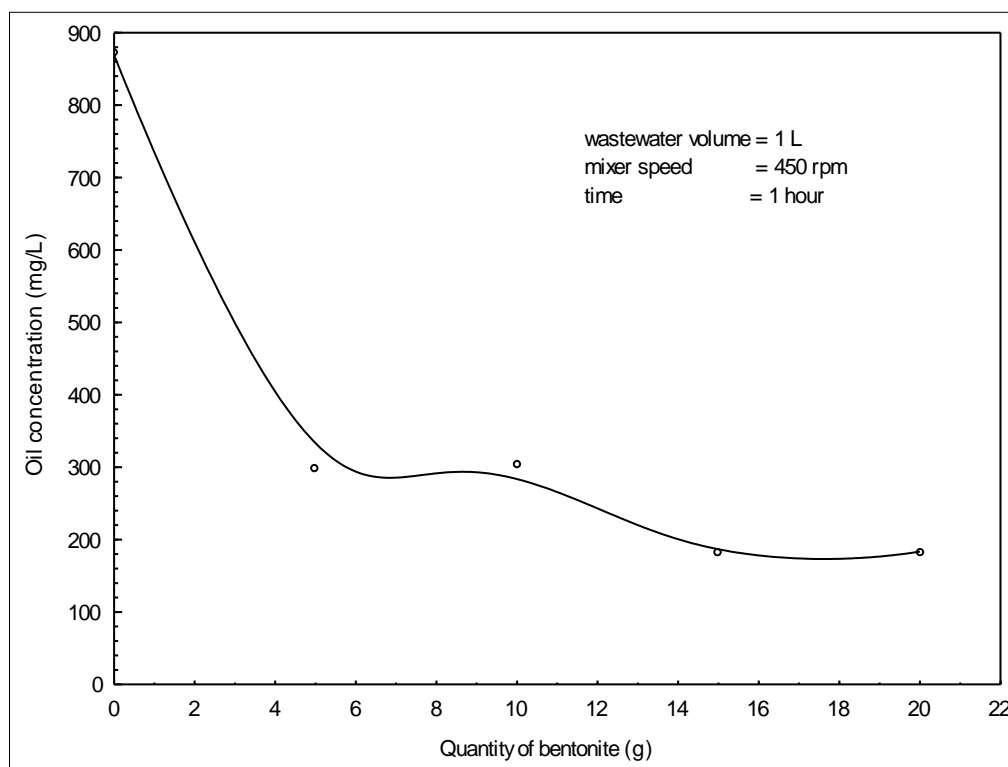
Fig. (5) Effect of bentonite quantity on oil concentration.
