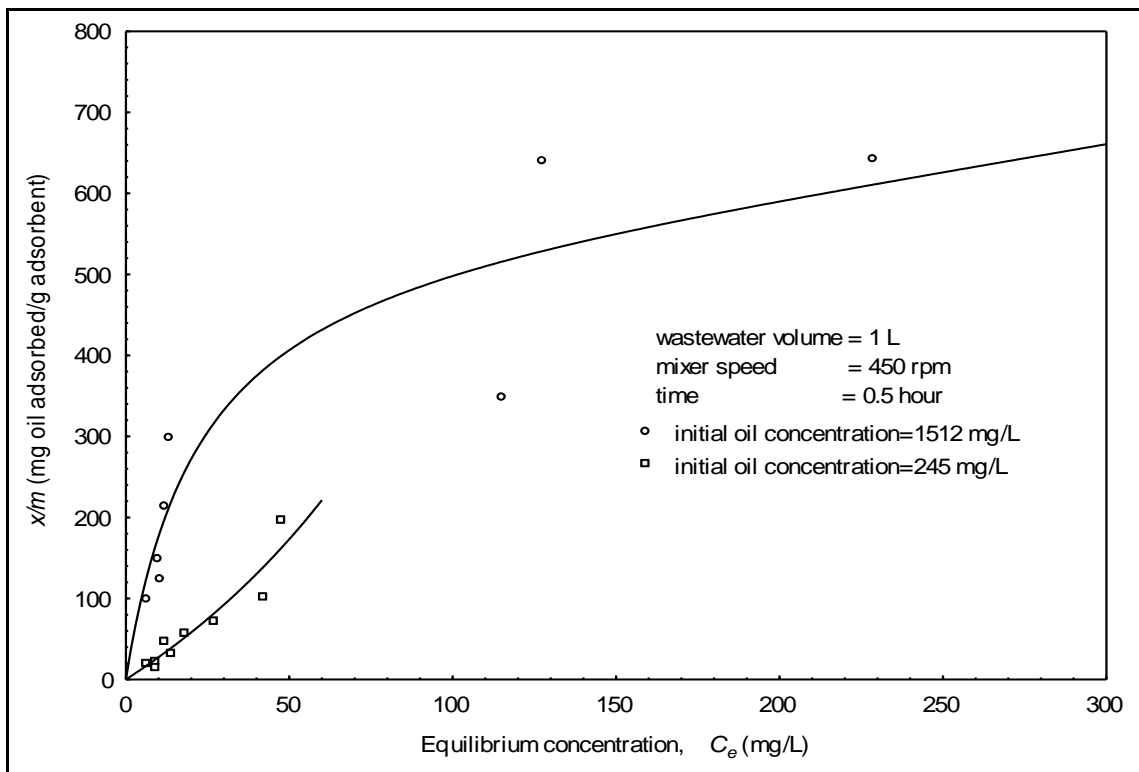
Fig. (18) BET isotherm for the adsorption of oil by organoclay
