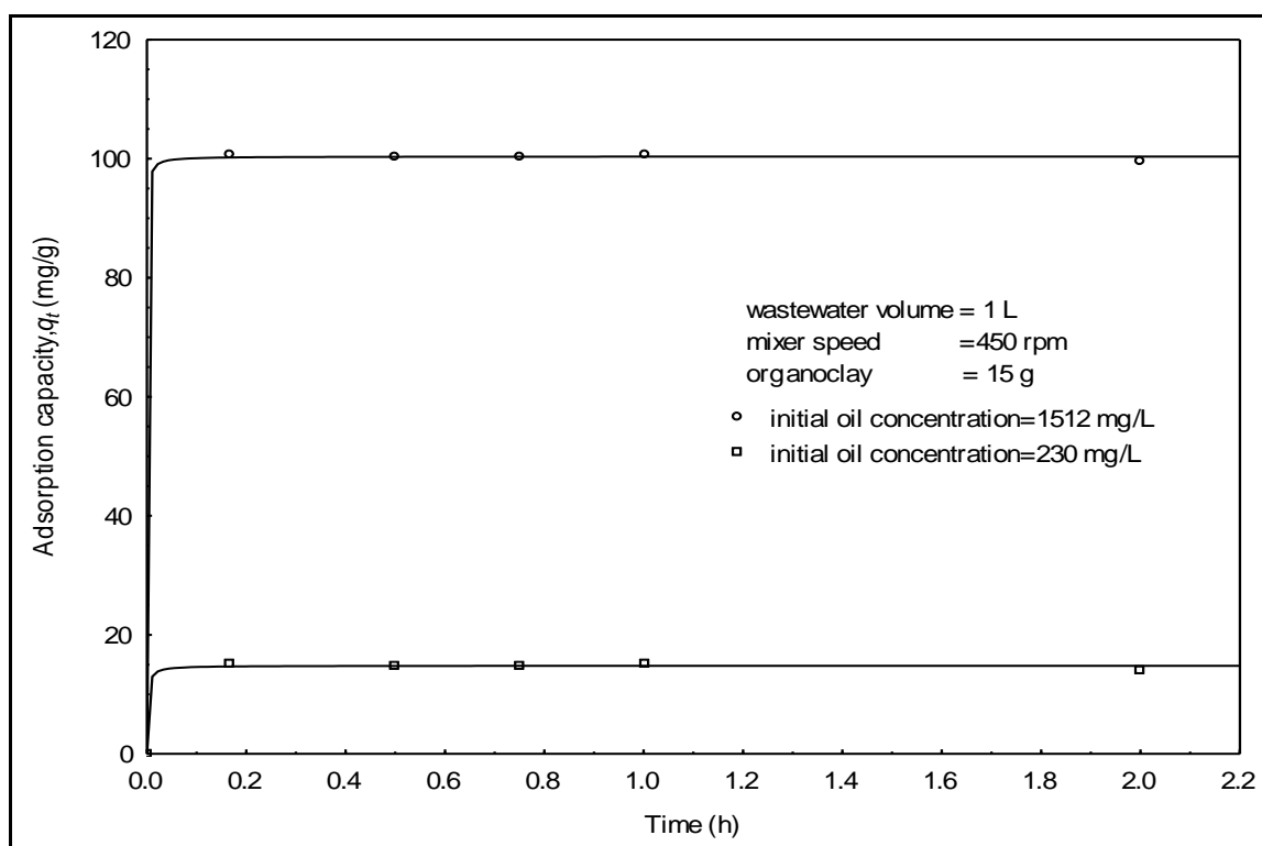
Fig. (15) Model of Ho et al. plot for the adsorption kinetics of oil by organoclay
