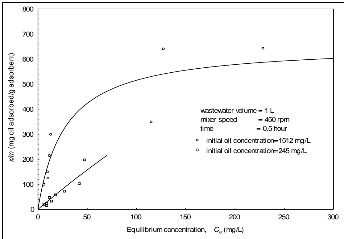
Fig. (17) Langmuir isotherm for the adsorption of oil by organoclay
