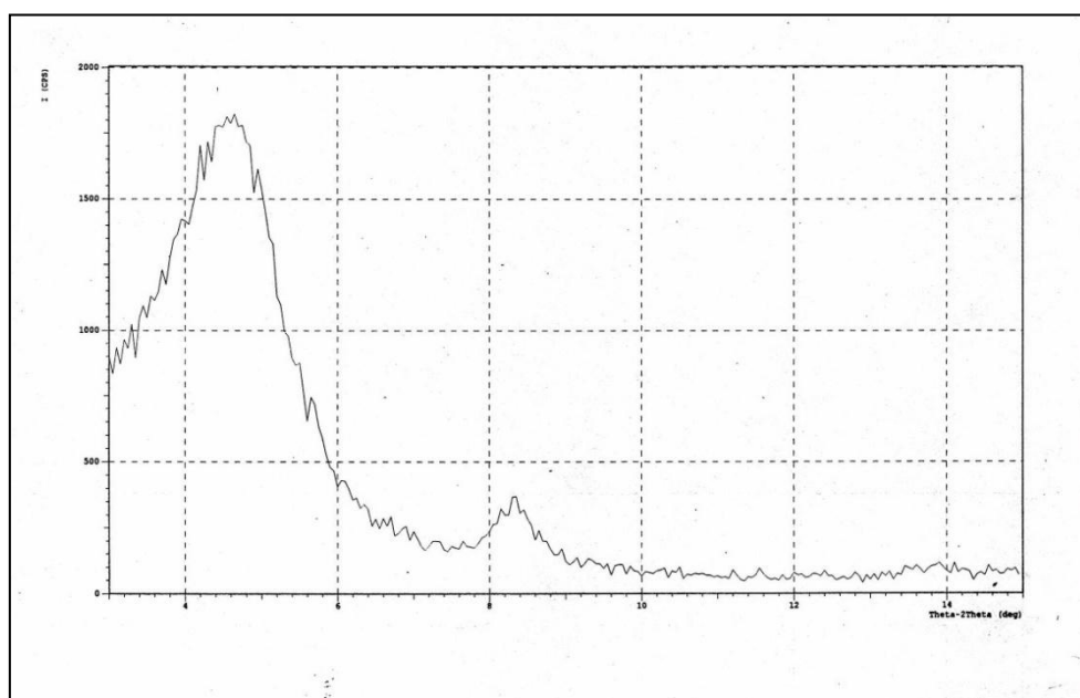
Fig. (2) XRD of prepared organoclay.
