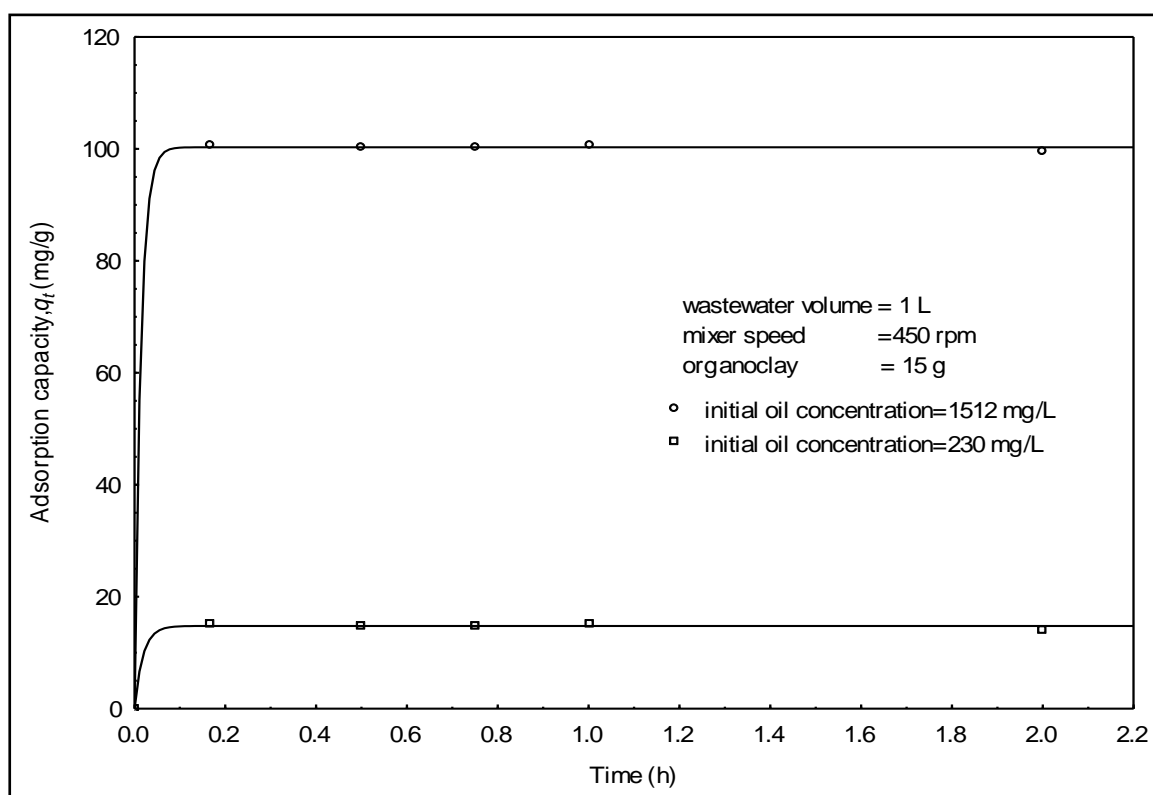
Fig. (14) Lagergren plot for the adsorption kinetics of oil by organoclay
