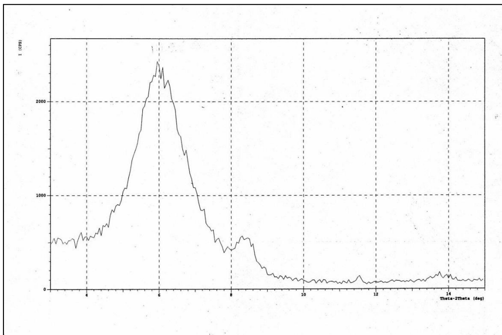
Fig. (1) XRD of natural Iraqi bentonite.
