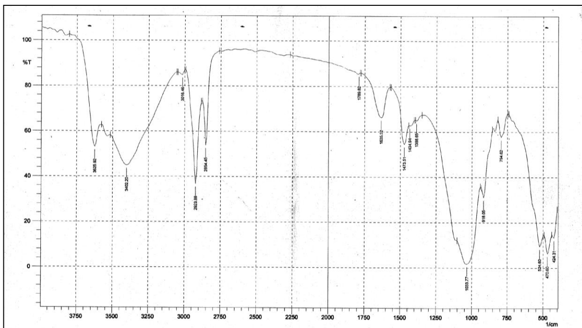
Fig. (4) Infrared curve of prepared organoclay.
