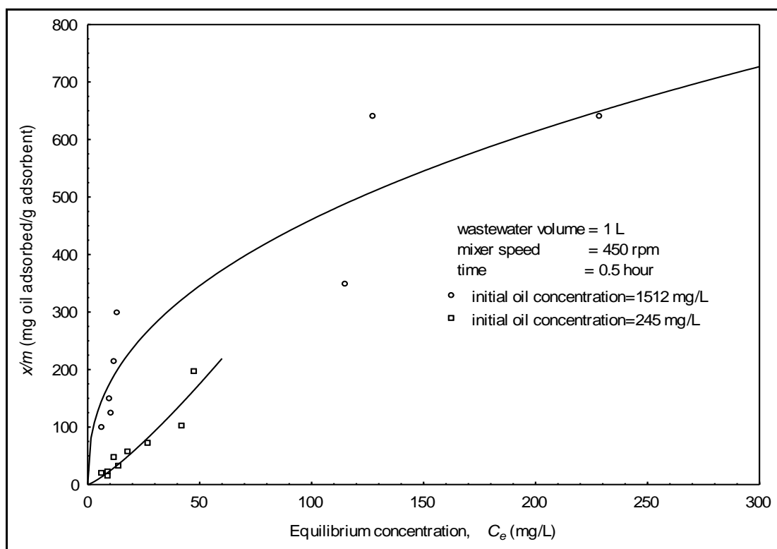
Fig. (16) Freundlich isotherm for the adsorption of oil by organoclay
