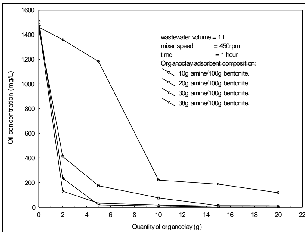
Fig. (6) Effect of organoclay quantity on oil concentration for different weight ratio of amine to bentonite ( C_o = 1450-1512\text{mg/L} ).
