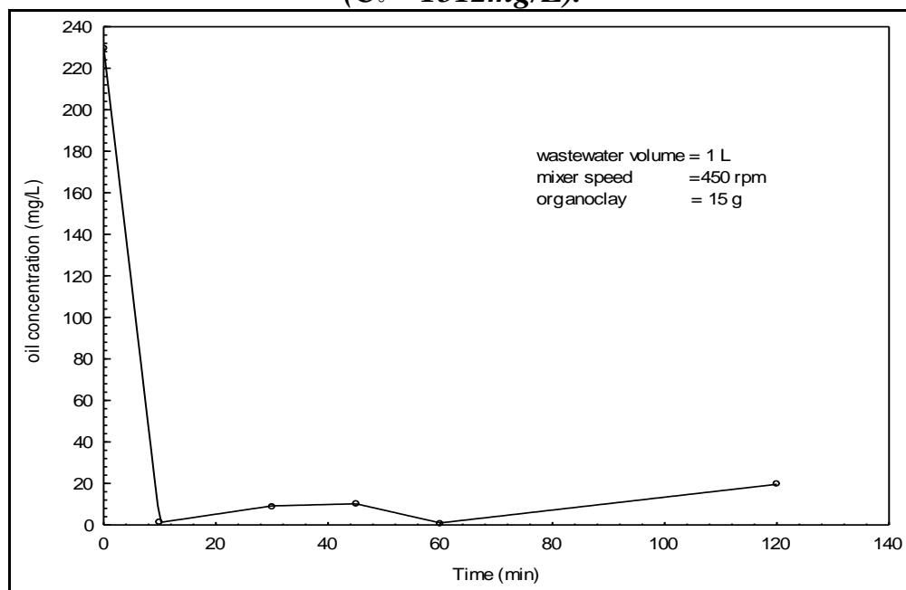
Fig. (12) Equilibrium time for the adsorption of oil by organoclay ( C_0 = 1512\text{mg/L} ).
