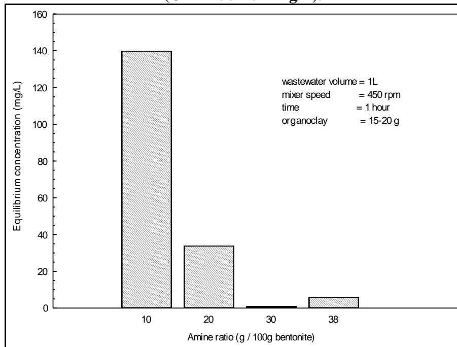
Fig. (9) Effect of amine to bentonite weight ratio on equilibrium concentration ( C_0 = 255-264\text{ mg/L} ).
