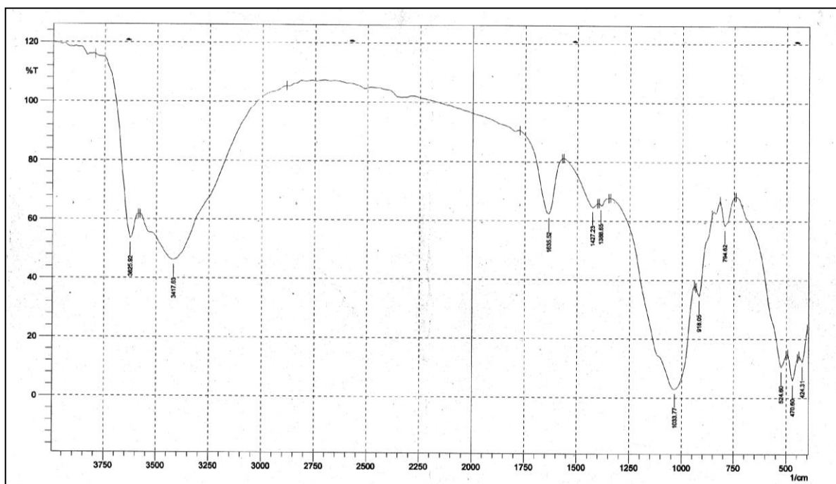
Fig.( 3) Infrared curve of natural Iraqi bentonite.
