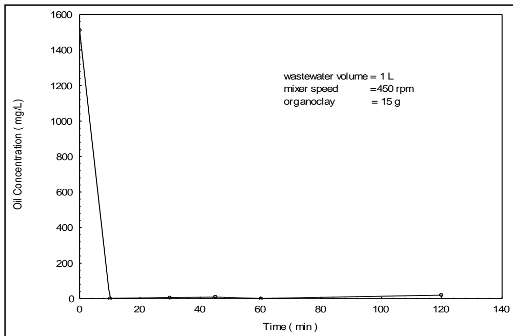
Fig. (12) Equilibrium time for the adsorption of oil by organoclay ( C_0 = 1512\text{mg/L} ).
