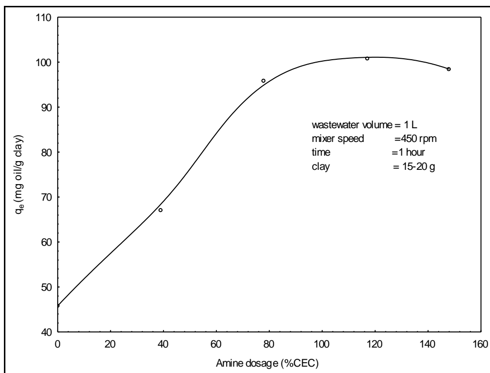
Fig. (10) Effect of amine dosage (%CEC) on adsorption capacity of organoclay ( C_o = 1450-1512\text{mg/L} ).
